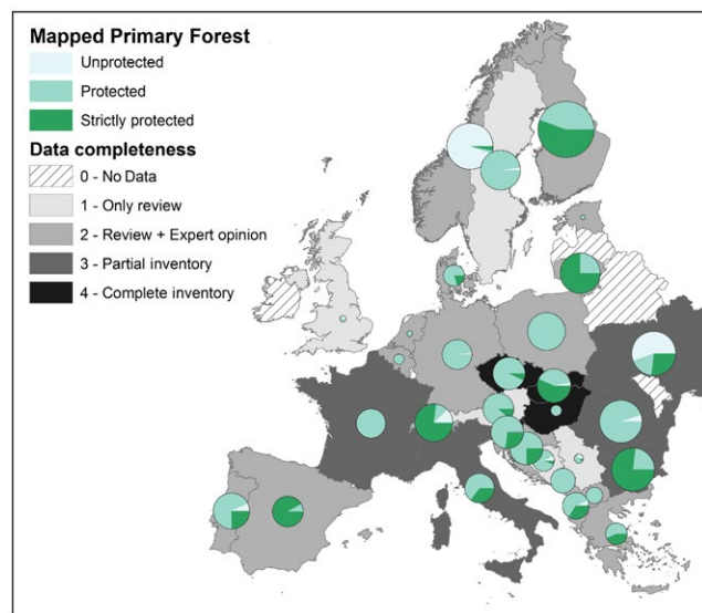
FIGURE 2 Contry-wise completeness of primary forest data and proportion of primary forest under strict protection (IUCN category I), included in protected areas having other IUCN categories or unprotected. The size of the pie is proportional to the logarithm of the total primary forest extent mapped in a country. The pie fractions only represent the data currently available and they should not be directly compared across countries, as data quality and availability differ. Furthermore, for some countries, only inventories of primary forest located either inside (e.g., Italy, Finland and France) or outside (Norway) protected areas were available [Colour figure can be viewed at wileyonlinelibrary.com ]
