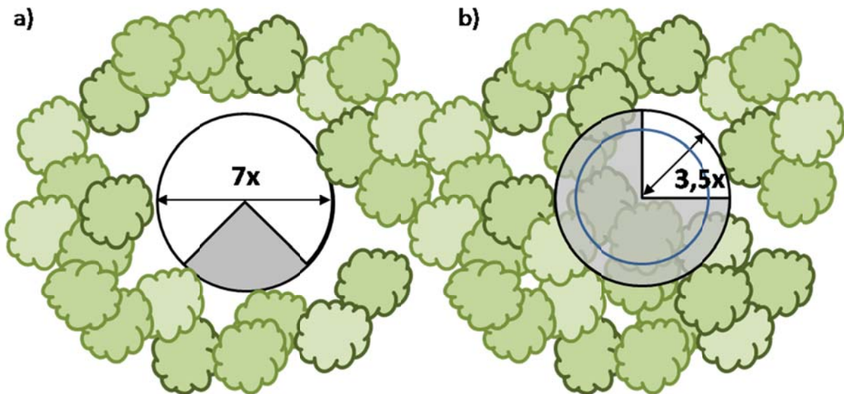
Fig. 5.21: A minimum clearing diameter of 7 times tree height is required for the full field of view (5 rings) without the use of viewcaps, while the use of larger viewcaps that cover three quarters of the sensor enables to use clearings with a minimum diameter of 3.5 times tree height
